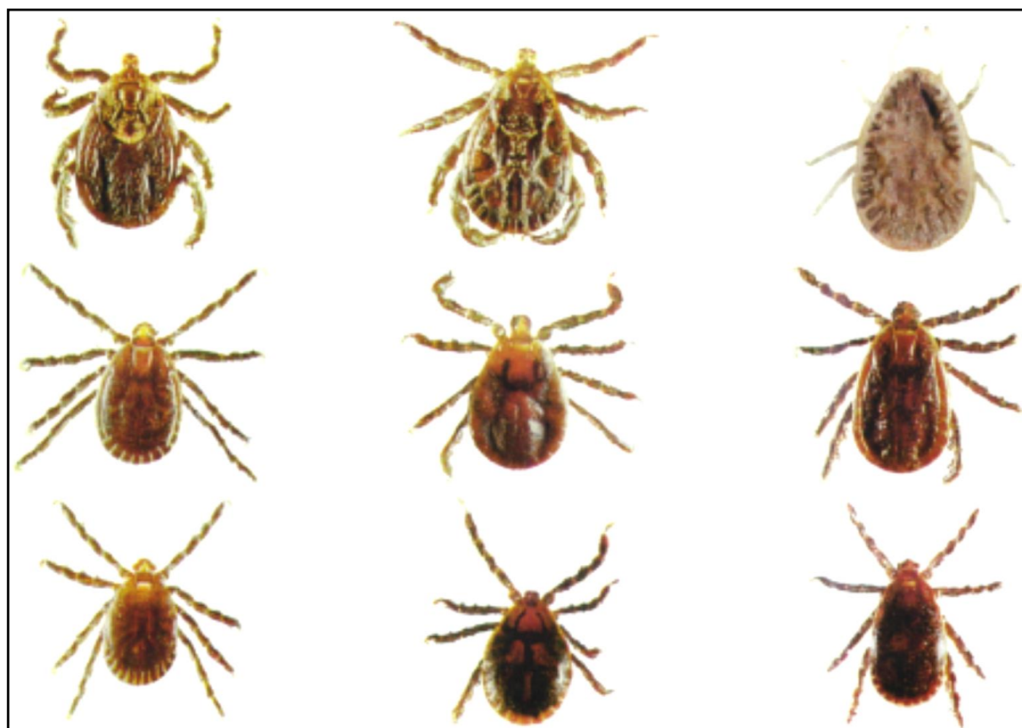
Dermacentor marginatus ♀ Haemaphysalis concinna ♀ Haemaphysalis concinna ♂
